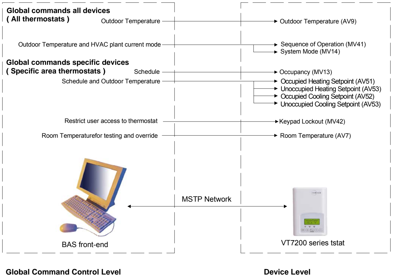
Figure 1: Global commands from a BAS front-end to a VT7200 series thermostat
